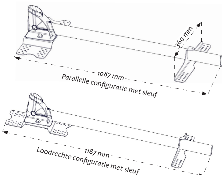
REF. 100543 Steunpoot.
